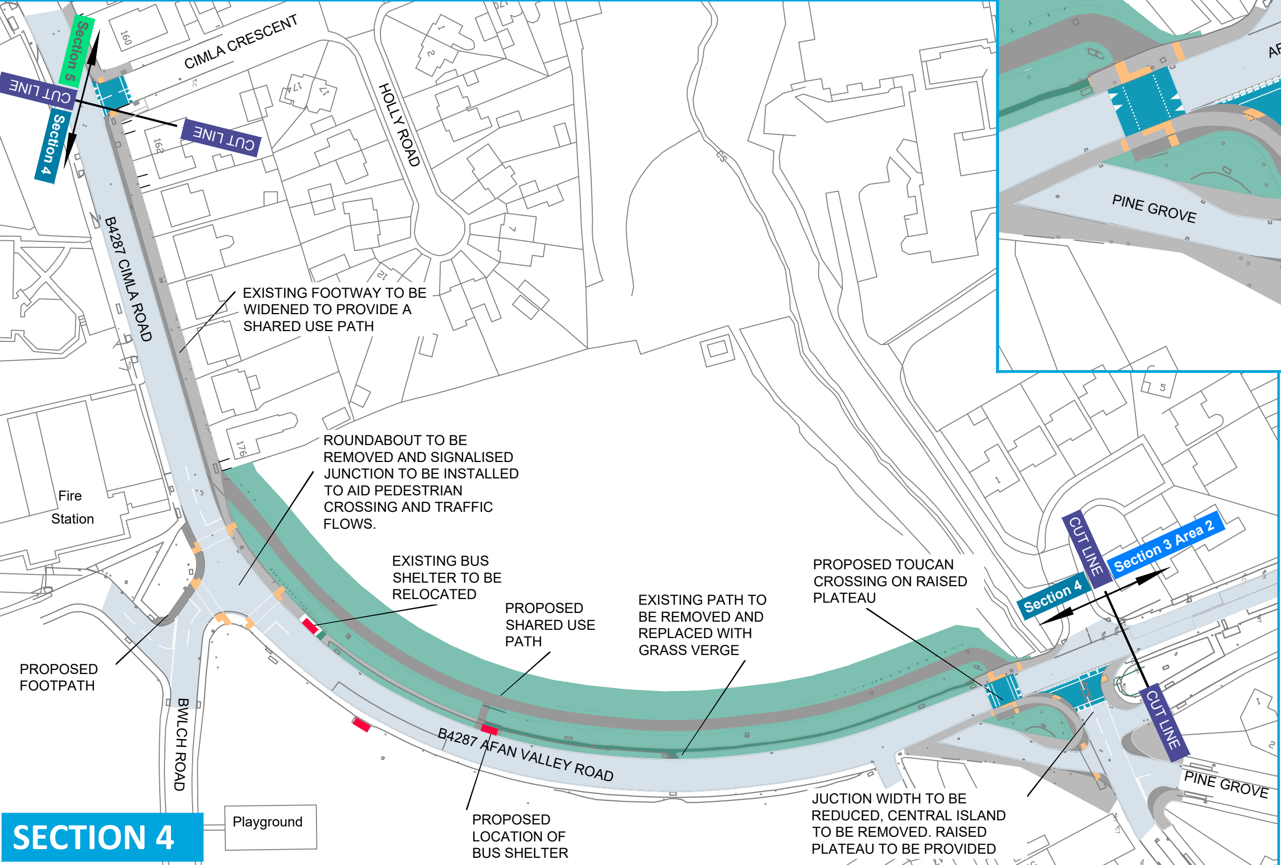
Enlarged detail of Afan Valley road Pine Grove junction.
